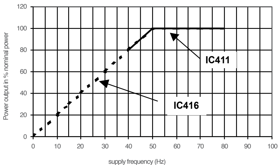
Diagram 2 Power output - supply frequency
