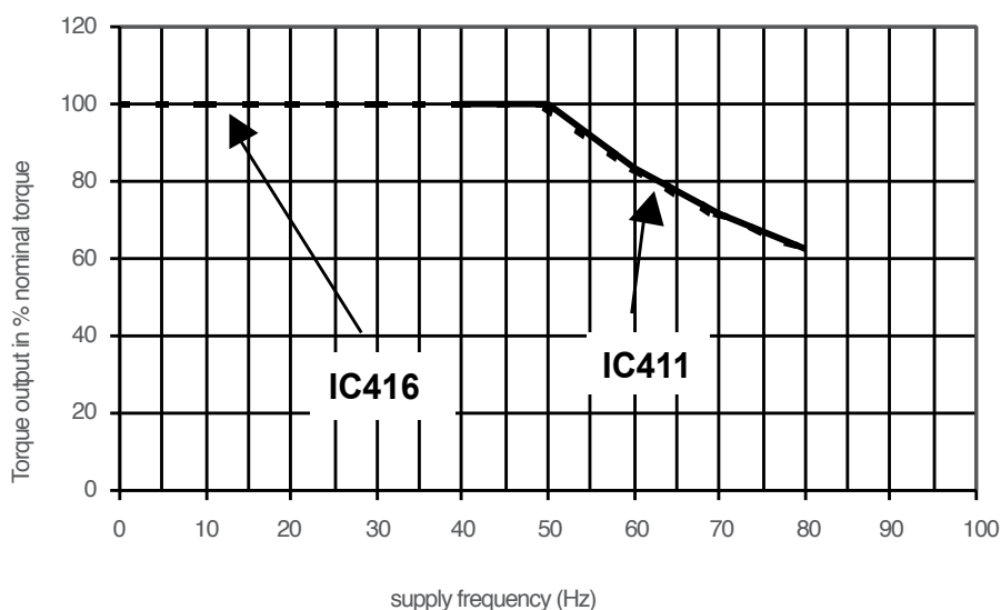
Diagram 3 Torque output - supply frequency
